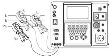
Current measurement with current clamps
