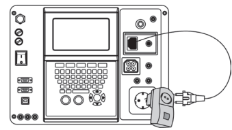
PRCD testing
