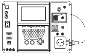
Polarity test
